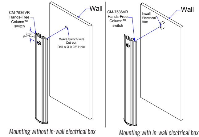
Figure 3.3 Wall Mounting Options
