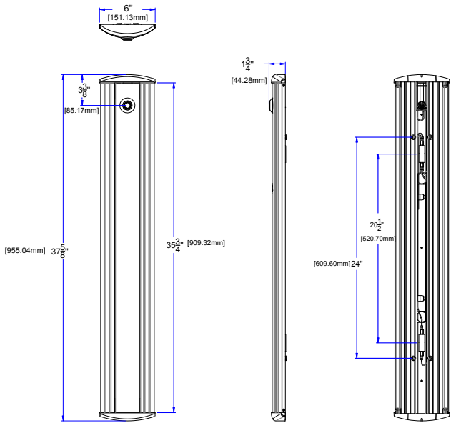
Figure 3.2 Dimensions
