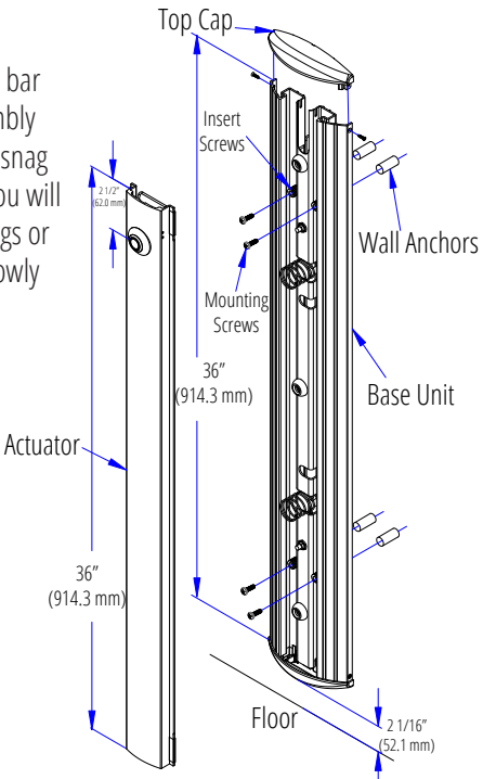
Figure 3.3 Mounting of Base Unit
