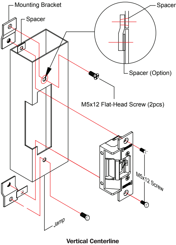
Figure 4.1 CX-ED2079 Strike Mounting
