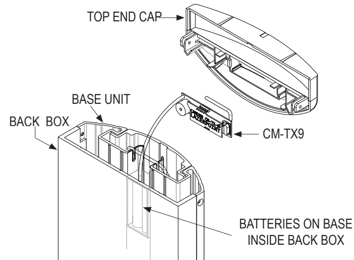
Figure 4.6 Transmitter Assembly
