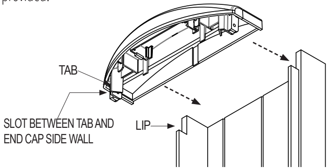
Figure 4.7 End Cap Alignment
