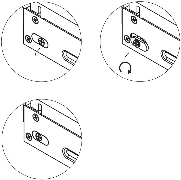
Figure 9.1 Fail Safe and Fail Secure Mechanism for CX-ED2079
