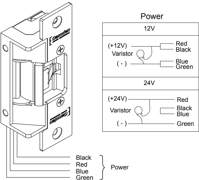
Figure 8.1 Connections for CX-ED2079
