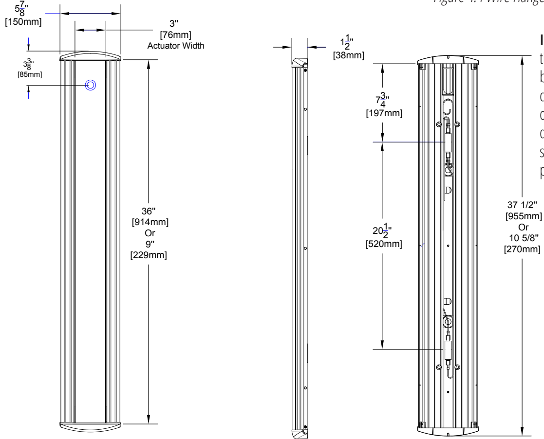
Figure 4.4 Wire Hanger/ End Cap
