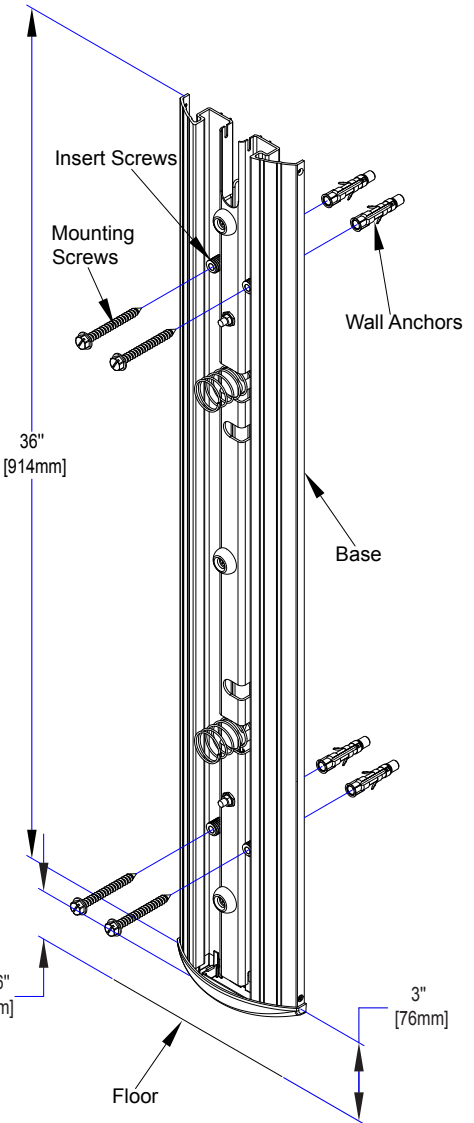
Figure 4.2 Mounting of Base Unit
