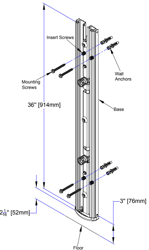
Figure 4.2 Mounting of Base Unit
