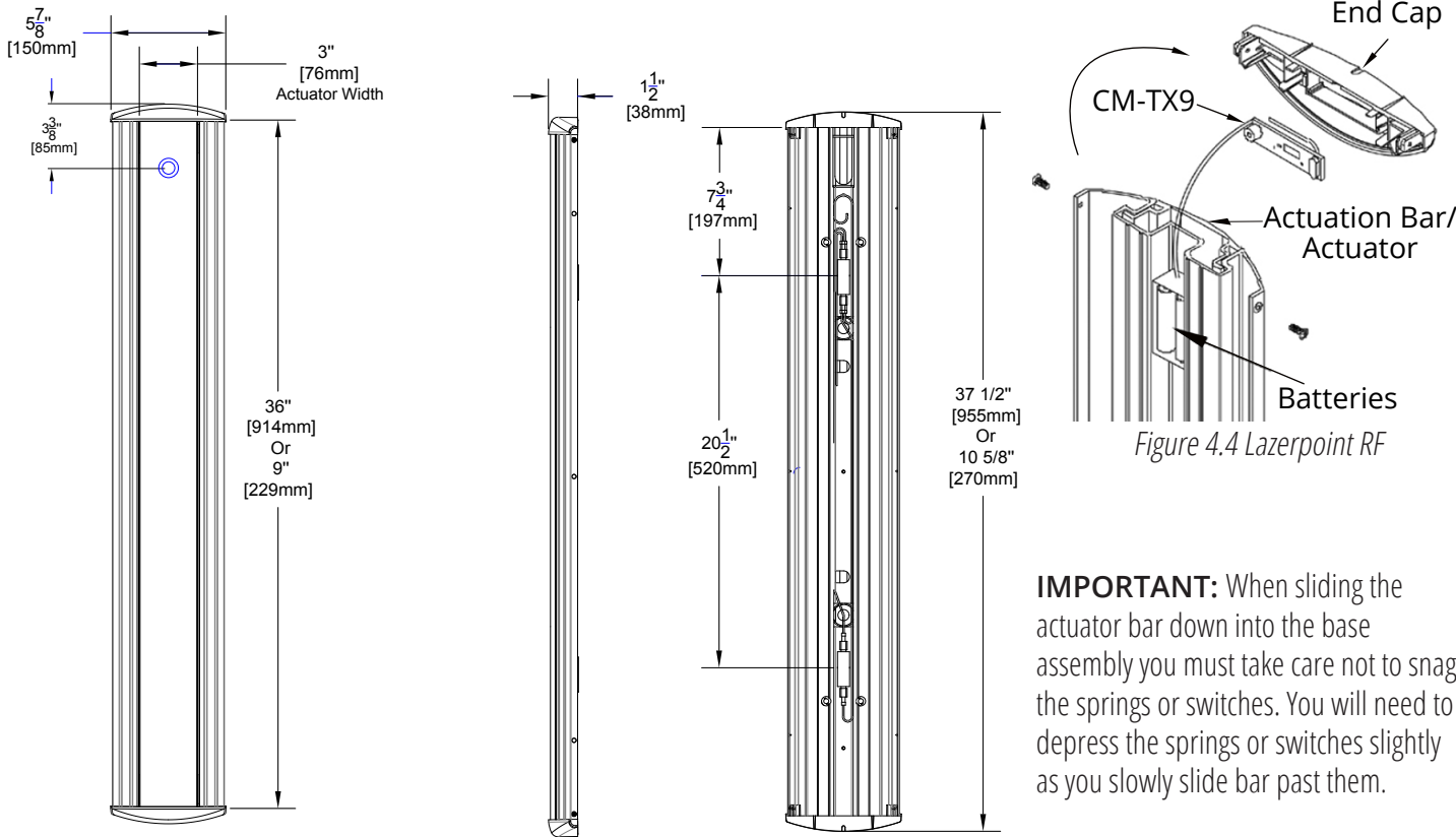
Figure 4.3 Dimensions
